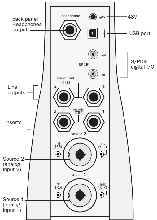
Figure 4. Mbox back panel
