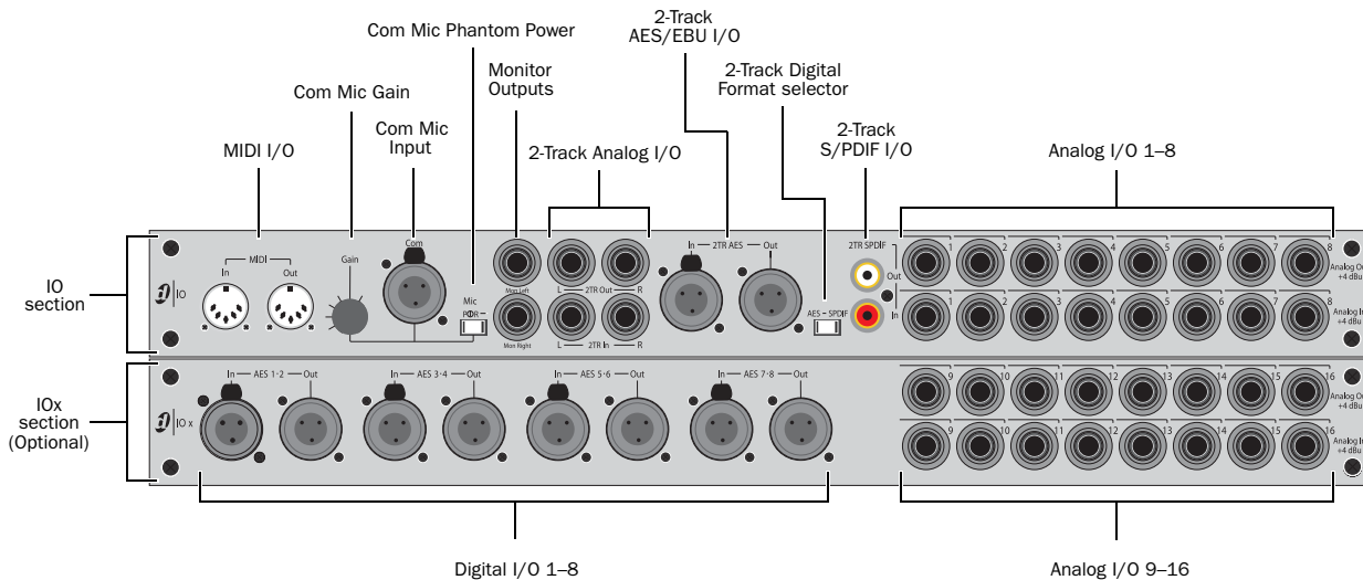
Figure 8. Audio connectors on FOH Rack, showing standard IO connectors (top) and optional IOx connectors (bottom)
