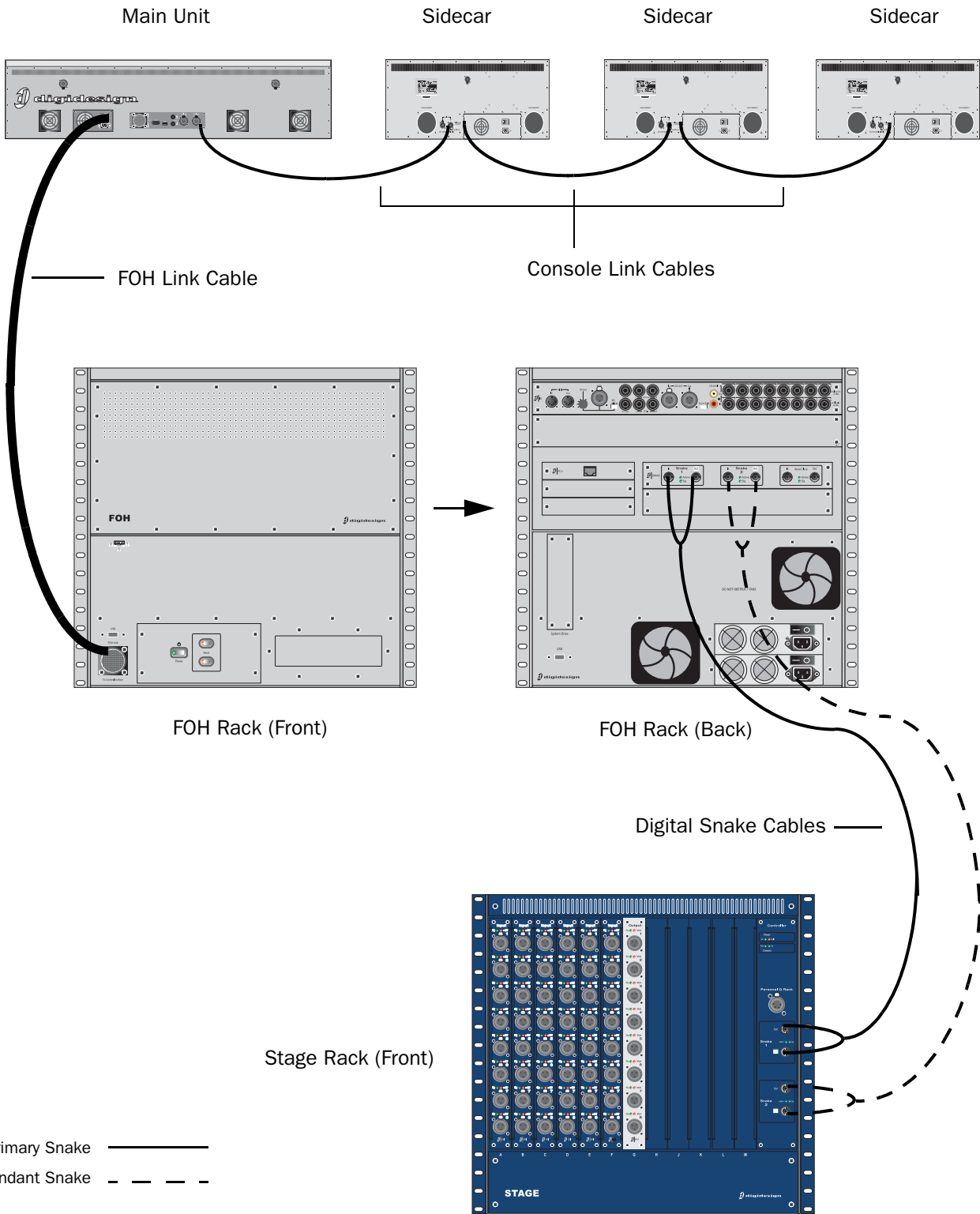
Figure 2. VENUE System system component connections
