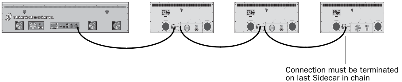
Figure 3. Console Link connections for Main Unit (left) and Sidecars (right)
