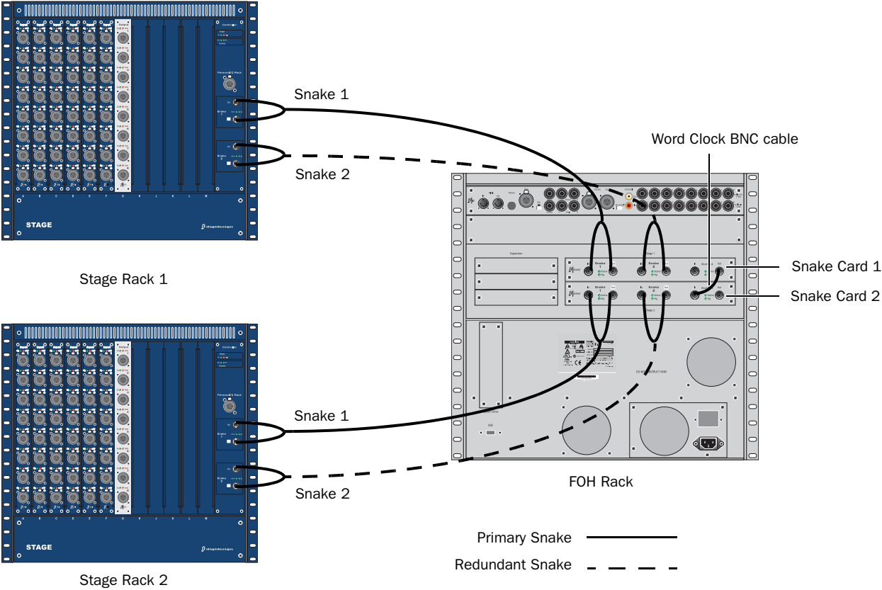
Figure 6. Digital Snake cable and word clock connections for fully redundant system with two Stage Racks
