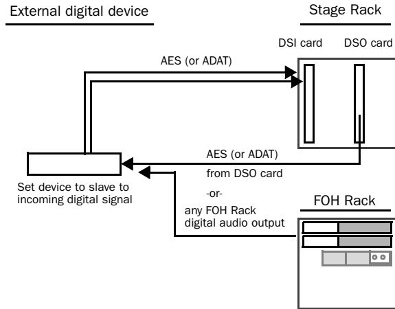
Using a digital output to provide clock to an external device
