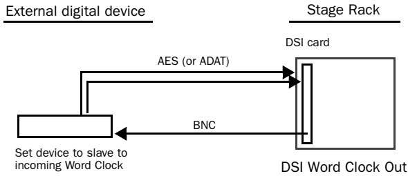
Using word clock from the DSI card to clock an external device
