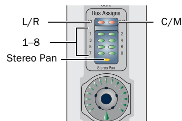
Input channel Bus Assign LEDs
