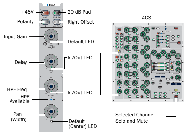
Input controls and their location in the ACS
