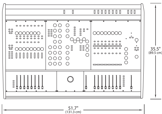
VENUE D-Show Main Unit dimensions
