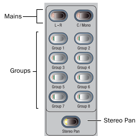
Bus Assign switches in the ACS
