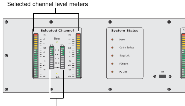
Selected channel gain reduction meters
