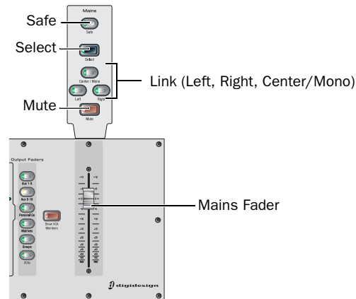
Mains Fader and controls in the Output section
