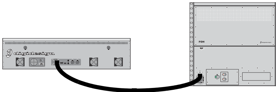
Figure 4. FOH Link connection between Main Unit (left) and FOH Rack (right)
