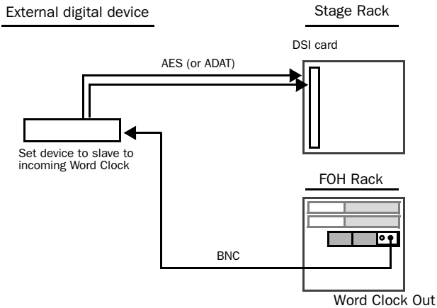
Using word clock from the FOH Rack to clock an external device
