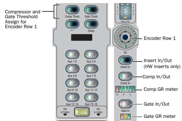
Dynamics controls and displays on input channels
