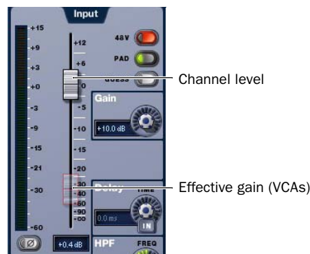
Effective gain (VCA contribution) shown on the selected channel
