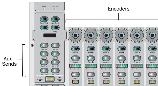
Aux assignment switches for input encoders
