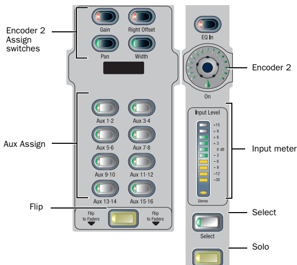
Input controls on input channel strips
