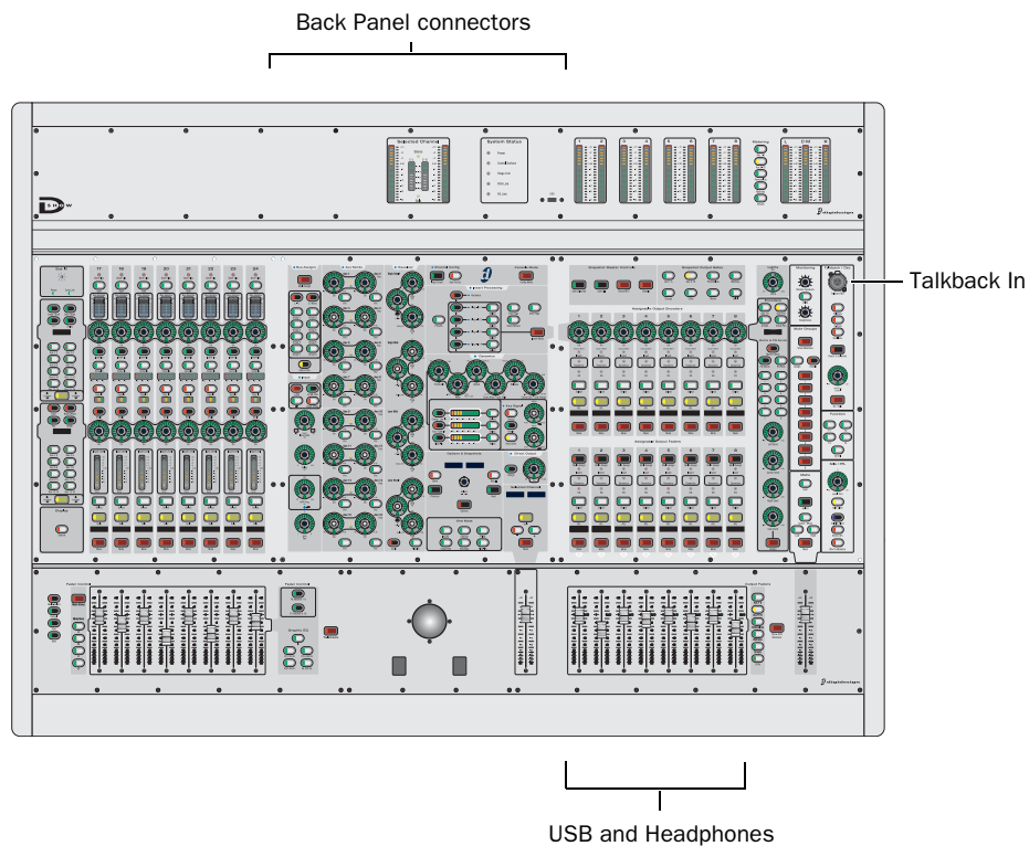
Figure 15. Main Unit top panel sections
