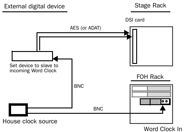
Using a distributed house (master) to clock a VENUE system and an external device
