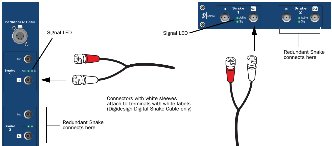
Figure 5. Detail of Digital Snake cable connection between Stage Rack (left) and FOH Rack (right)
