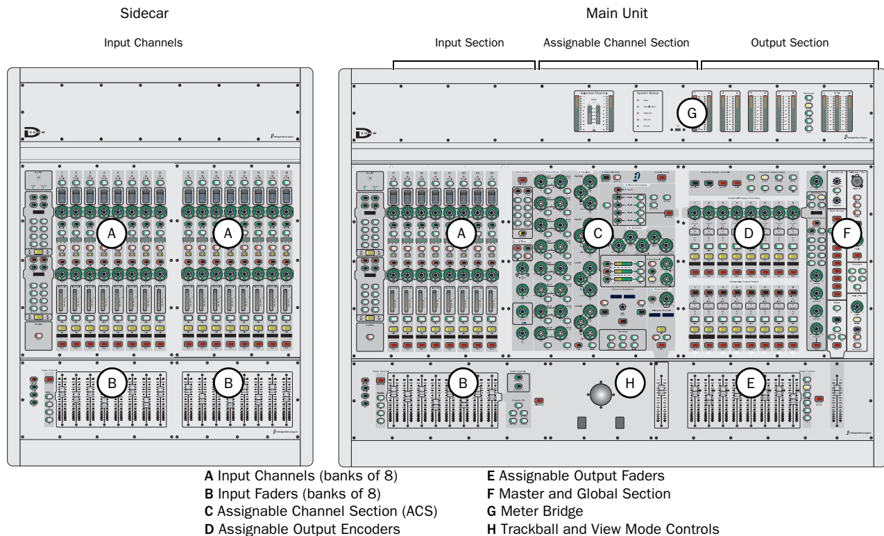
Figure 9. Control Surface main sections
