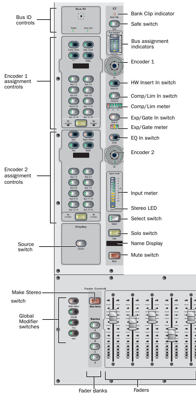
Input strip and fader controls
