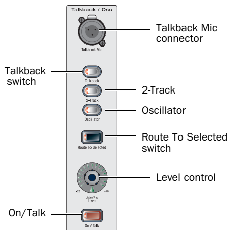
Talkback controls in the Talkback/Osc section
