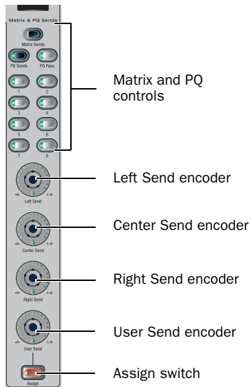
Matrix and PQ mixer controls
