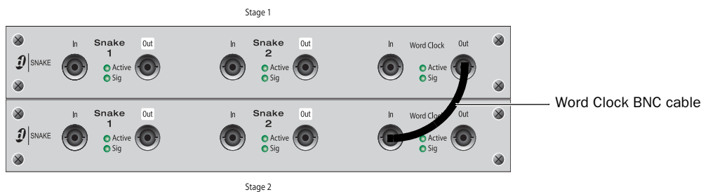
Word Clock connection between Snake cards
