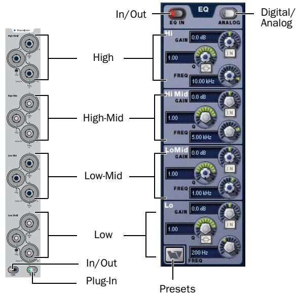
EQ controls in the ACS (left) and on-screen (right) for an Input Channel FX Returns provide two bands of EQ (Hi and Lo) which can be toggled between Bell and Shelf modes.
